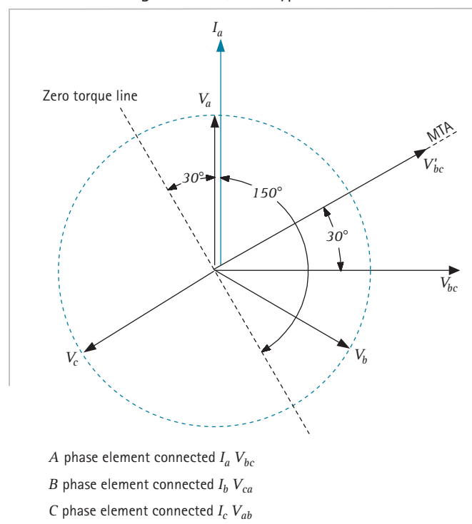
Figure 9.11: Vector diagram for the 90°-30° connection (phase A element)
