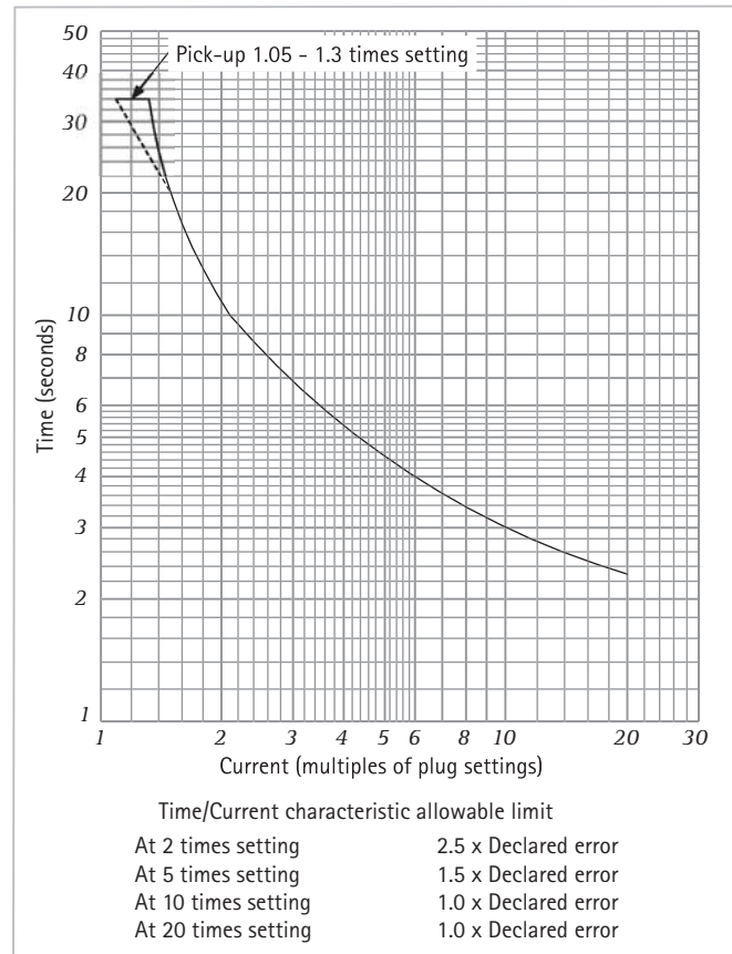
Figure 9.10: Typical limits of accuracy from IEC 60255-4 for an inverse definite minimum time overcurrent relay
